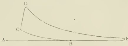
Fig. 5.—Indicator-diagram of Atkinson's Engine.
