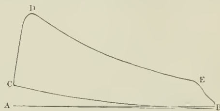
Fig. 3.—Indicator-diagram of Otto's Engine.
